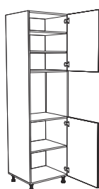
IN MDF D60 RV 60 x 57 x 222 cm ID KD 60RV**
