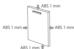
FRONTOVI KANTOVANI SA 4 STRANE 18 mm univer, sa ABS-om 1 mm. Four side edge banding of front doors 18 mm chipboard, with ABS 1 mm.
